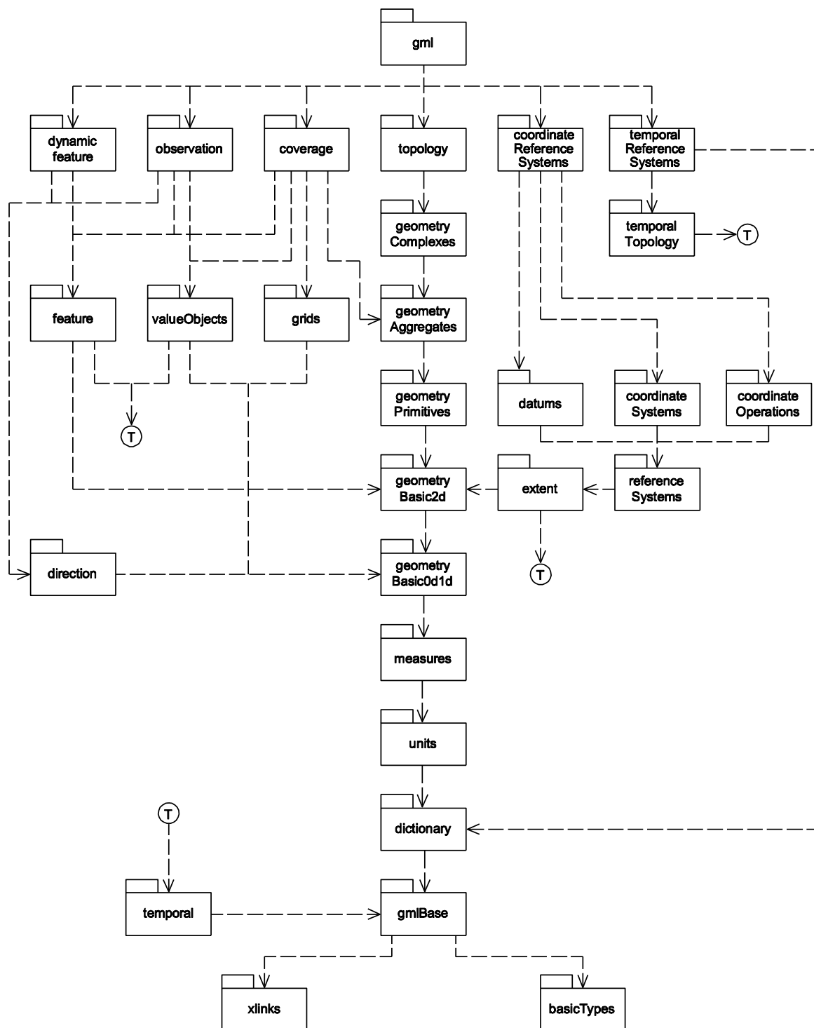
Figure 82 — Schema dependencies
