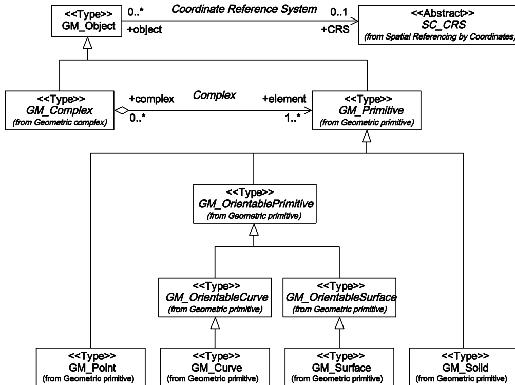
Figure 10 — Geometric primitives
