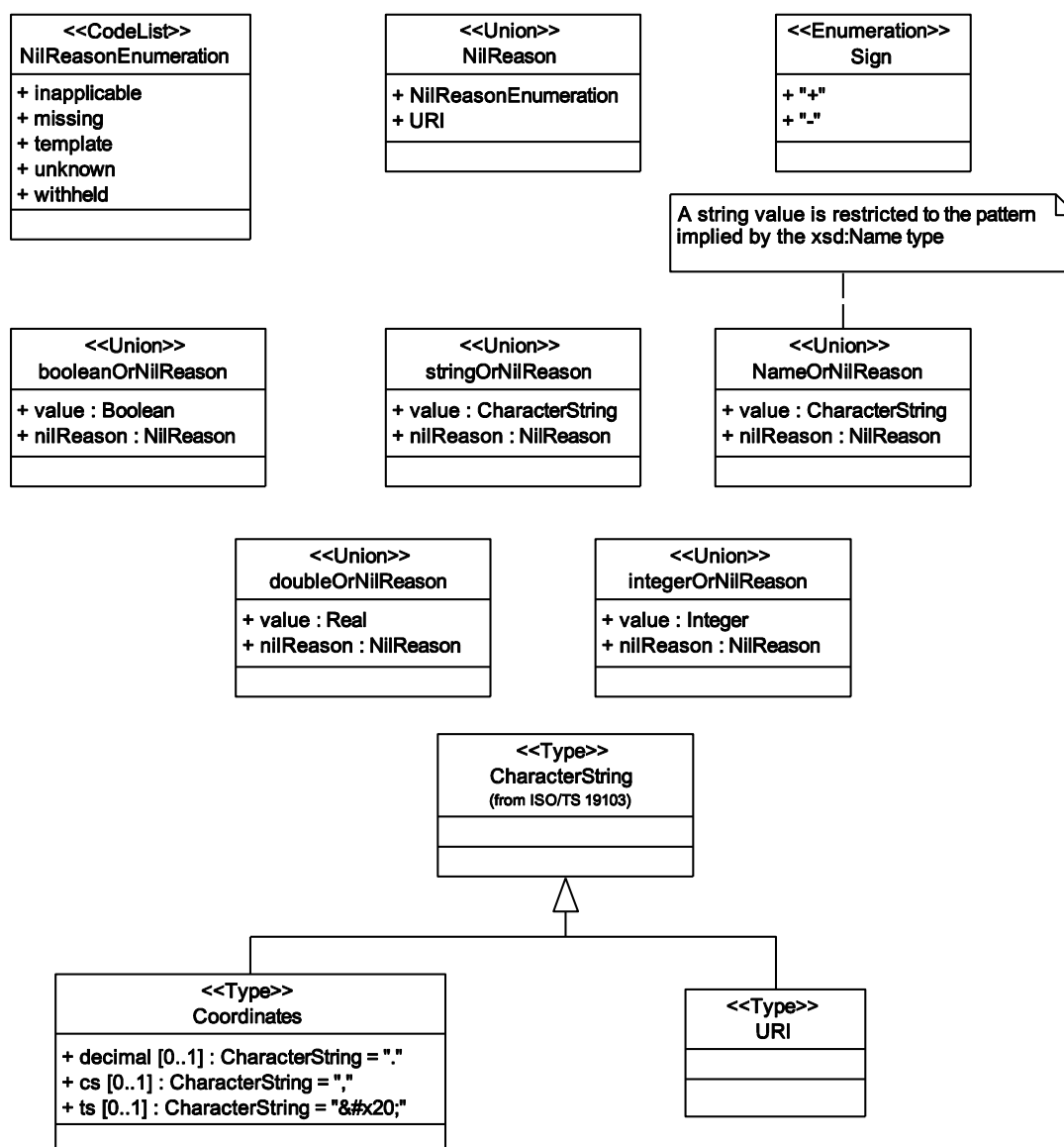
Figure 49 — Simple types
