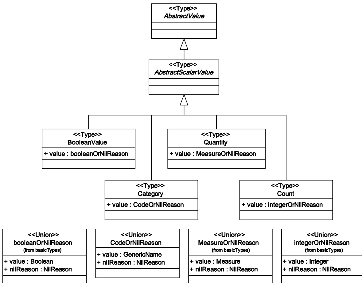
Figure 69 — Scalar values
