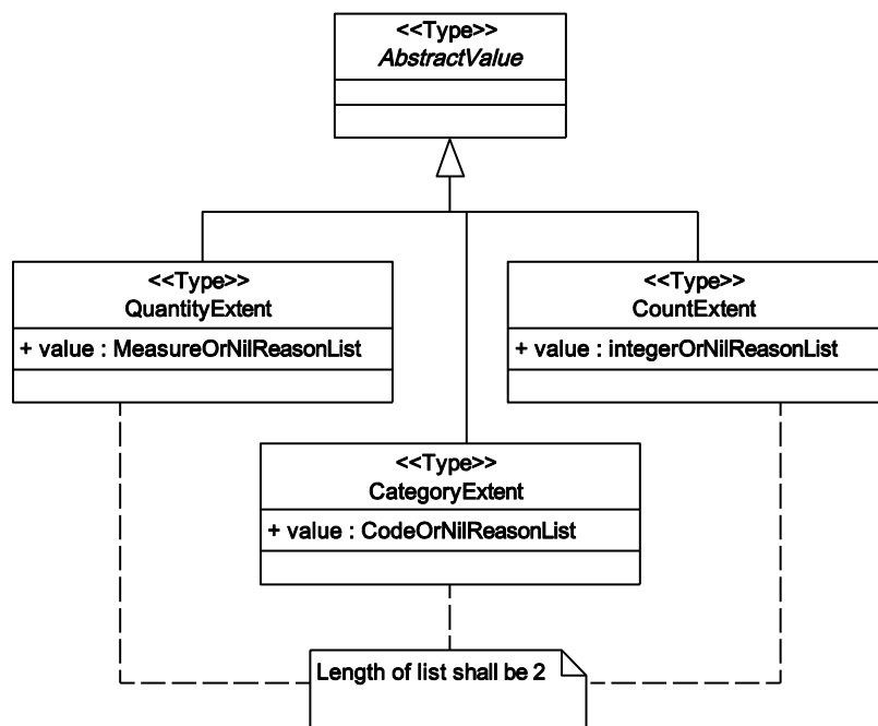
Figure 72 — Extents
