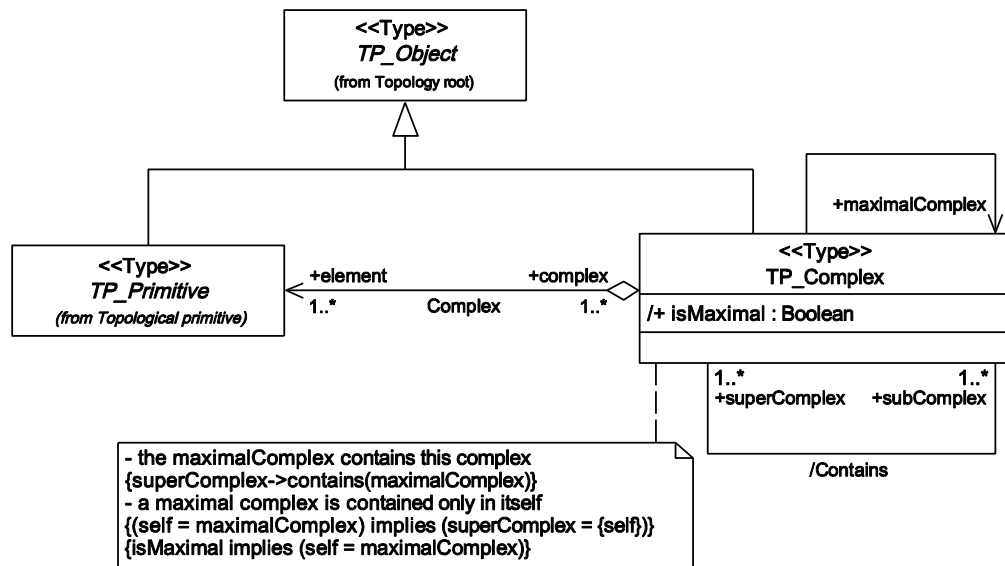
Figure 37 — Topology complex
