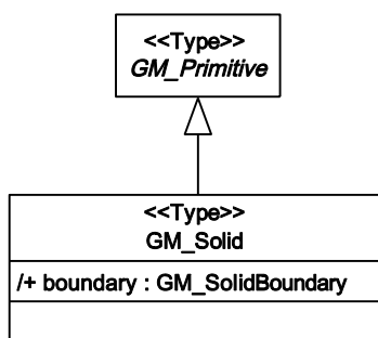
Figure 17 — Solid
