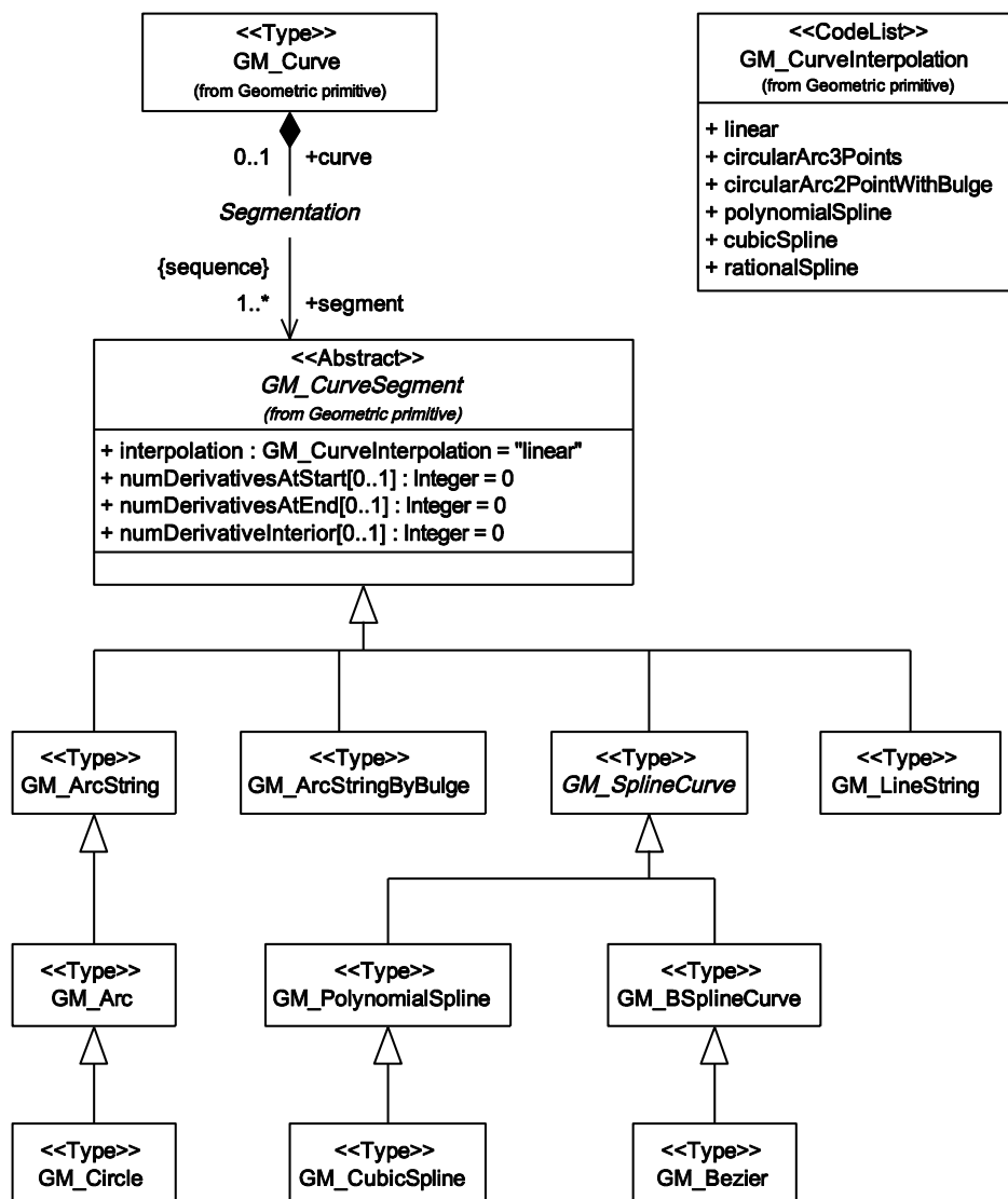
Figure 19 — Curve segments
