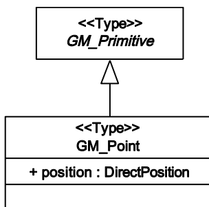
Figure 13 — Point
