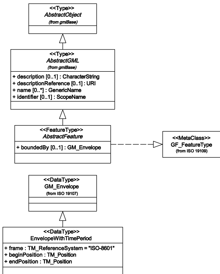
Figure 53 — Features
