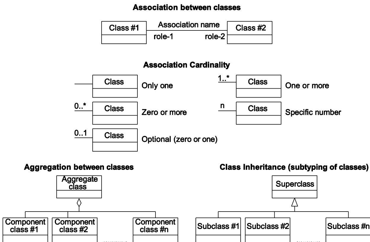
Figure 1 — UML notation
