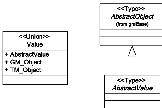
Figure 68 — Value expressions
