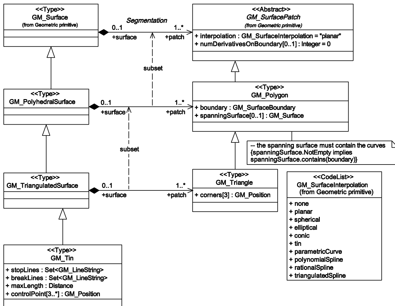
Figure 27 — Polyhedral and triangulated surfaces
