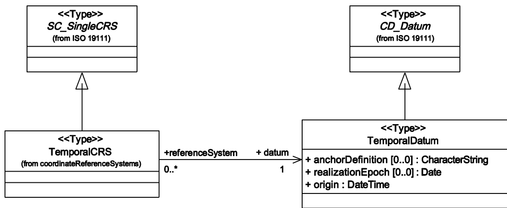
Figure 62 — Association between TemporalCRS and TemporalDatum
