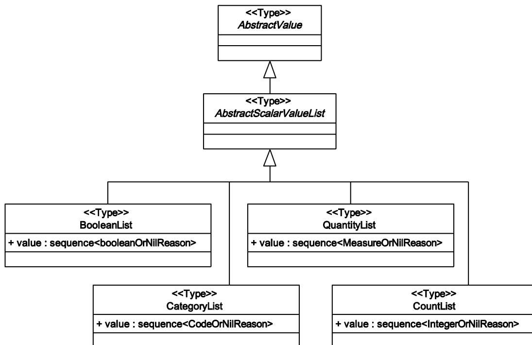
Figure 70 — Scalar value lists
