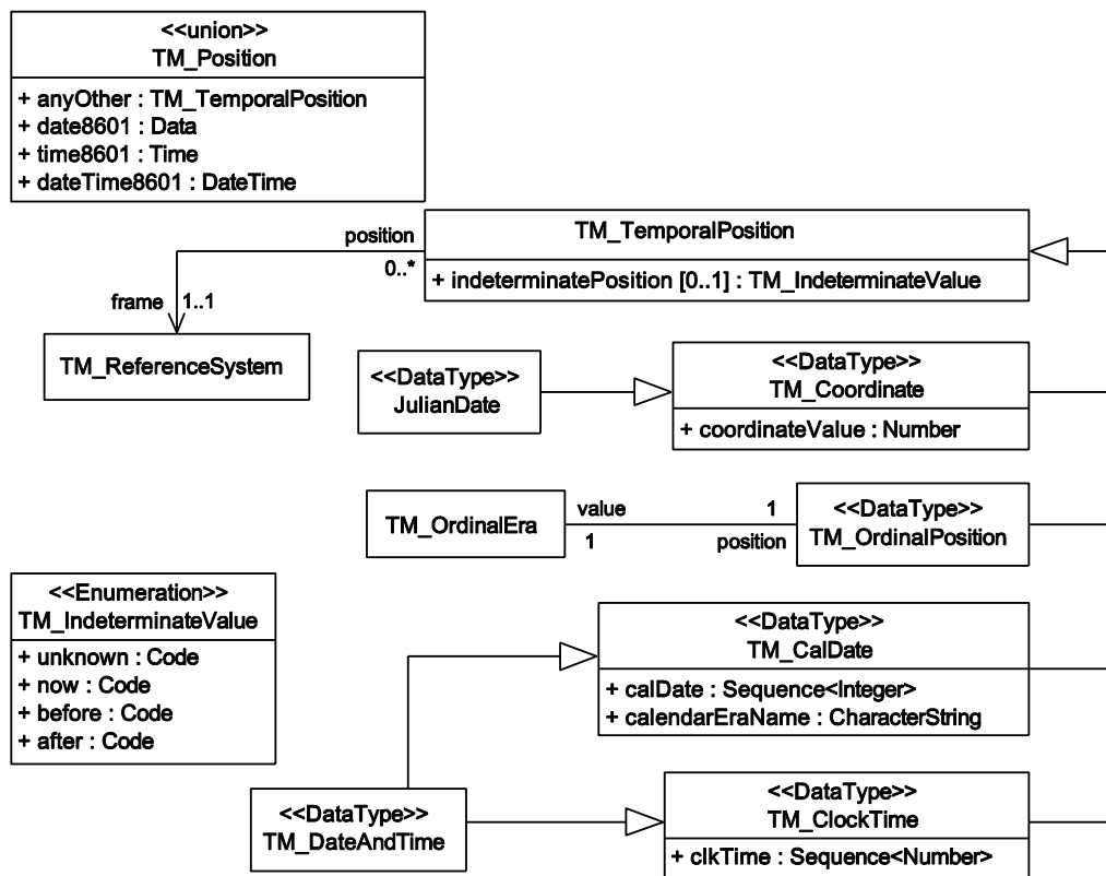
Figure 41 — Temporal position, from ISO 19108
