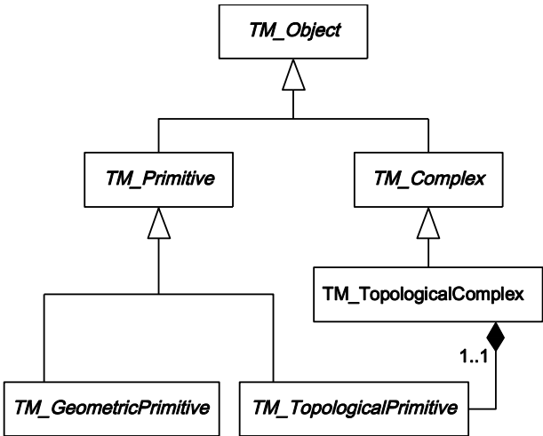
Figure 38 — Main hierarchy of temporal objects from ISO 19108
