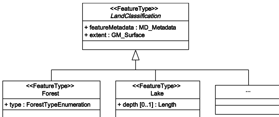
Figure 79 — Generalization relationship between feature types <informative>
