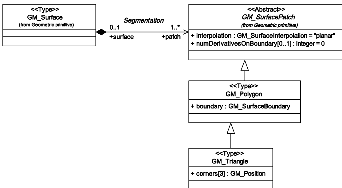
Figure 25 — Surface patches (second figure)
