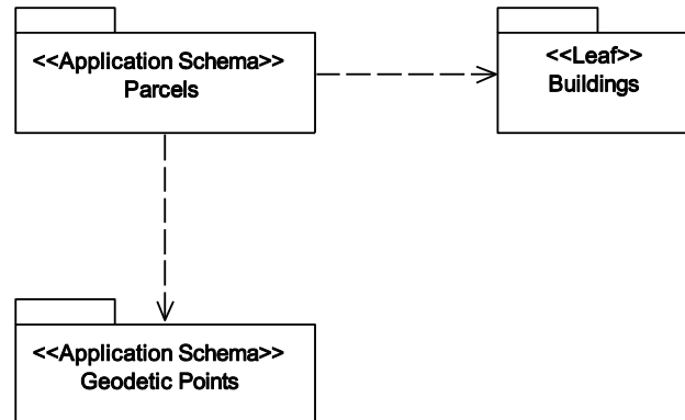
Figure 75 — Dependency between packages <informative>
