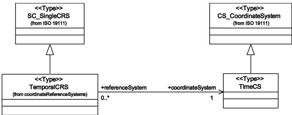
Figure 60 — Association between TemporalCRS and TimeCS
