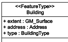
Figure 76 — A feature type &lt;informative&gt;
