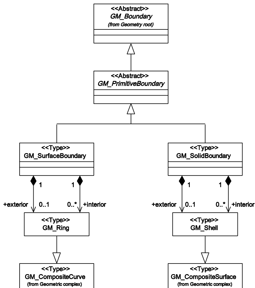
Figure 11 — Boundaries of geometric primitives
