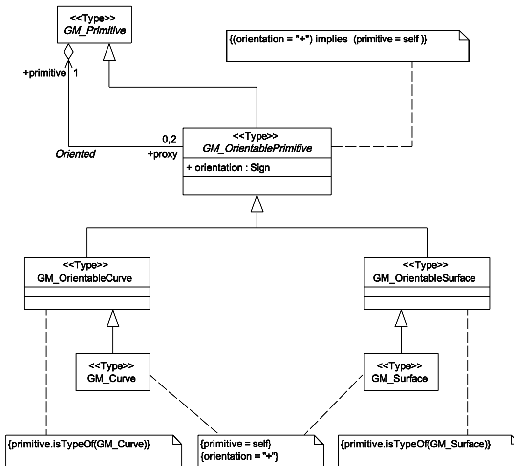
Figure 14 — Curve and Surface
