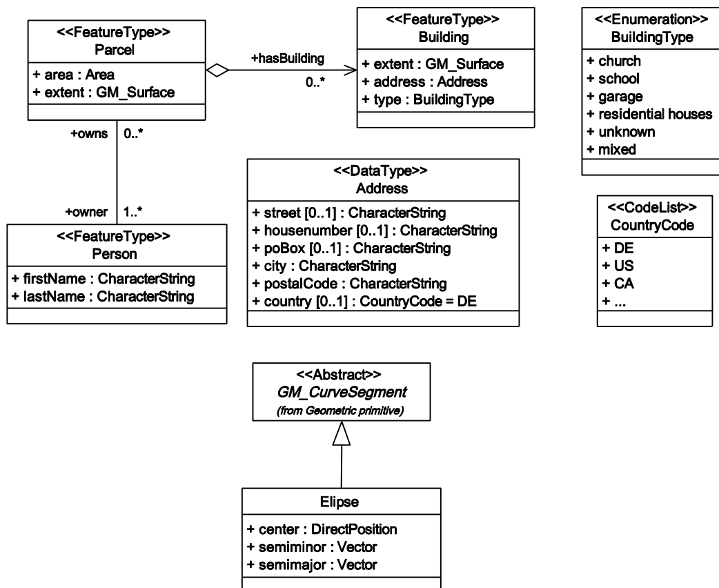
Figure 81 — Example application schema
