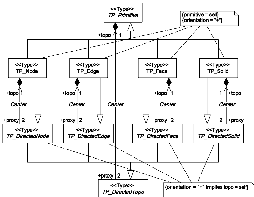
Figure 35 — Directed Topology primitives
