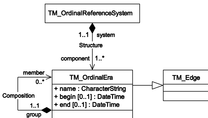
Figure 46 — Model for temporal ordinal reference system, adapted from ISO 19108
