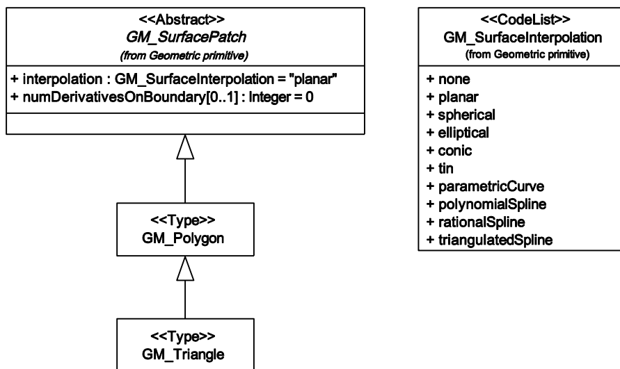
Figure 24 — Surface patches (first figure)
