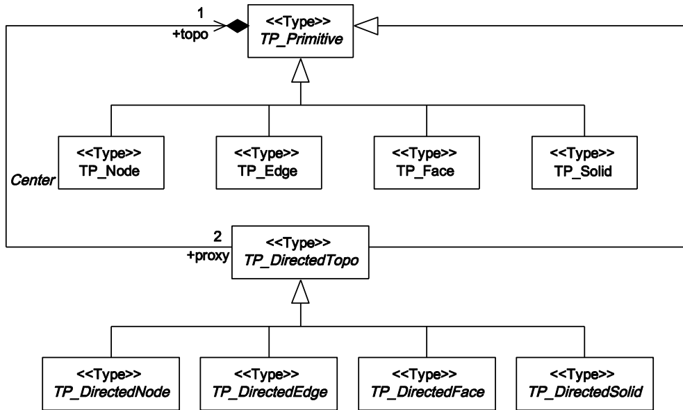
Figure 34 — Topology primitives
