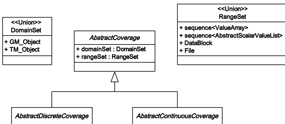
Figure 47 — Coverages overview
