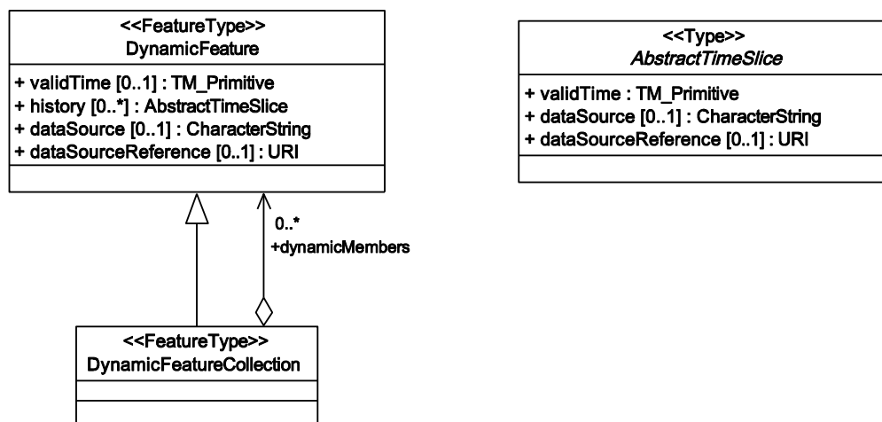
Figure 64 — Dynamic features
