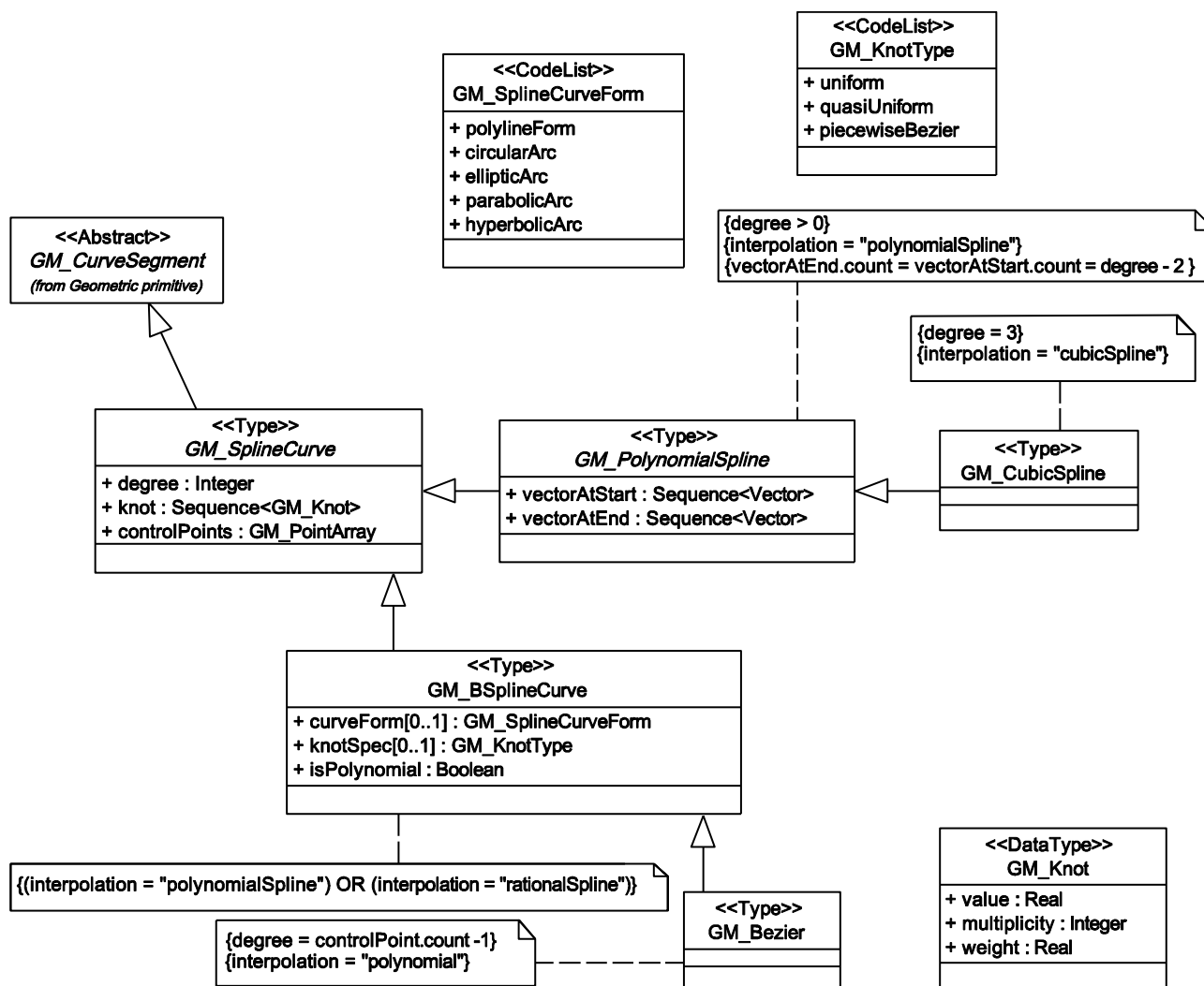
Figure 22 — Splines
