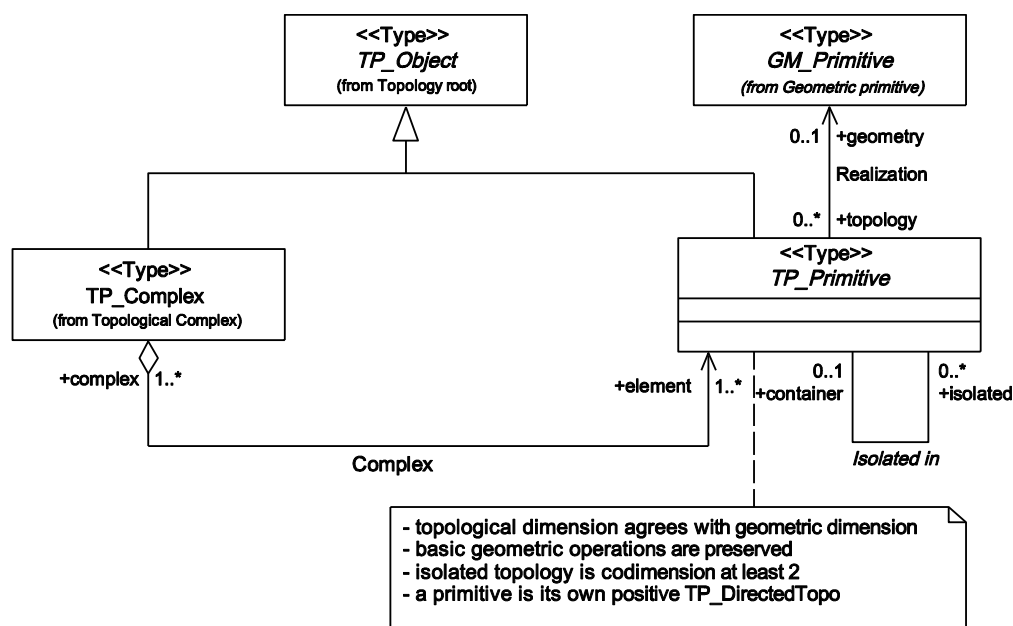
Figure 33 — Topology primitive
