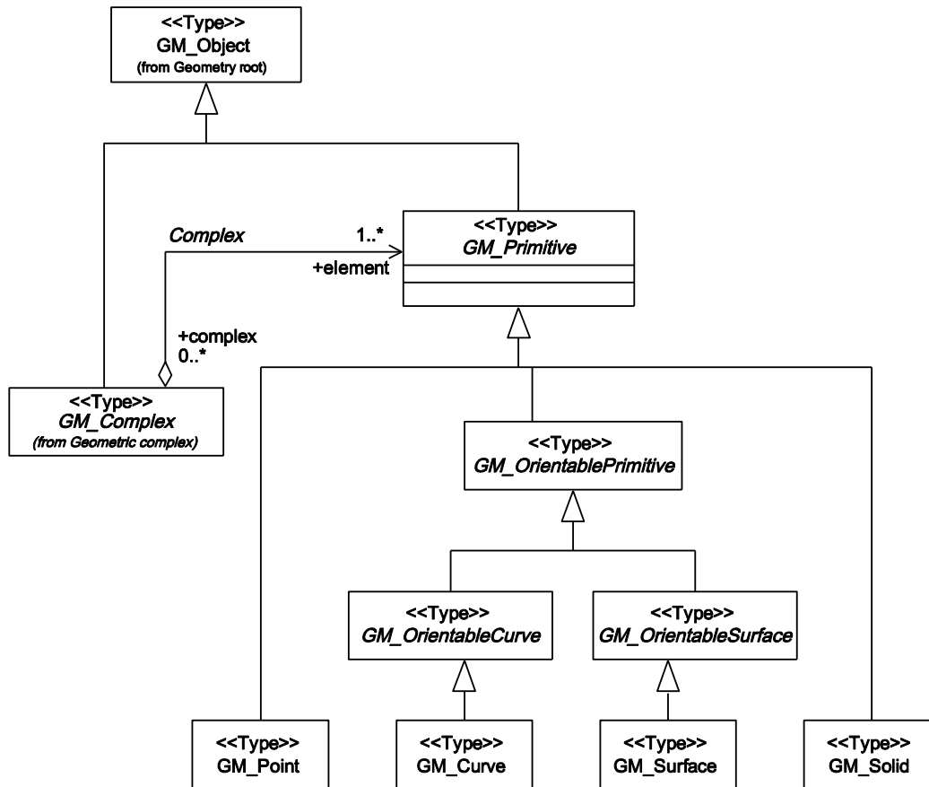
Figure 12 — Geometric primitives
