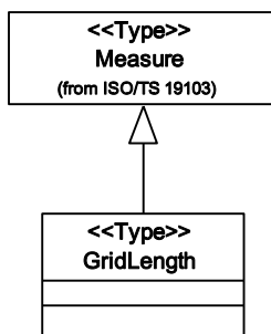
Figure 67 — Additional measures
