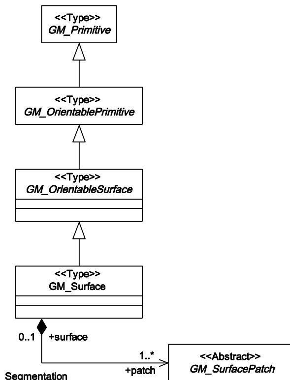
Figure 16 — Surface
