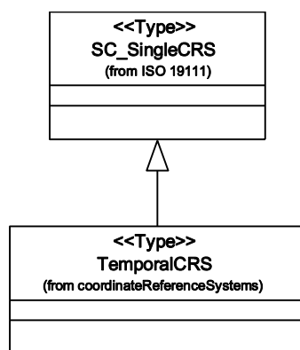
Figure 58 — TemporalCRS
