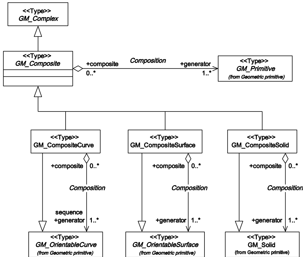
Figure 30 — Geometric composites (second figure)
