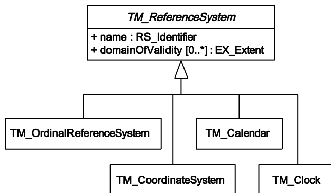
Figure 43 — Hierarchy of temporal reference systems from ISO 19108
