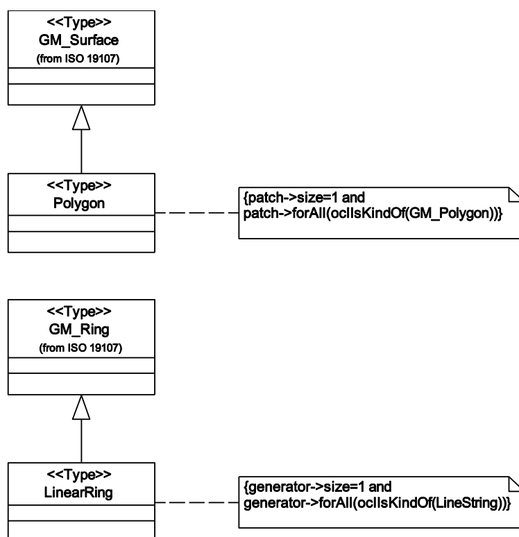
Figure 55 — A GM_Surface with a single GM_Polygon patch
