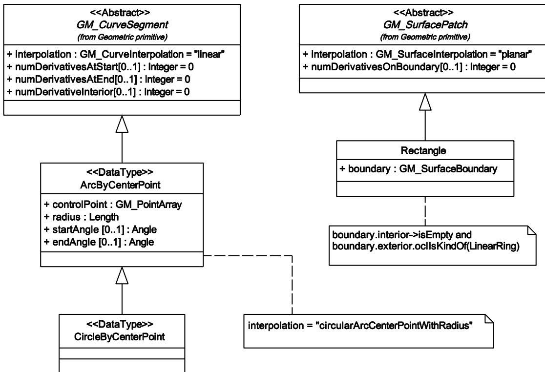
Figure 56 — Additional curve segments and surface patches
