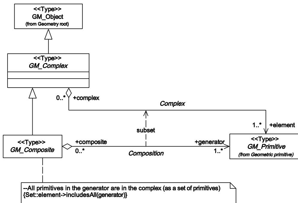
Figure 29 — Geometric composites (first figure)
