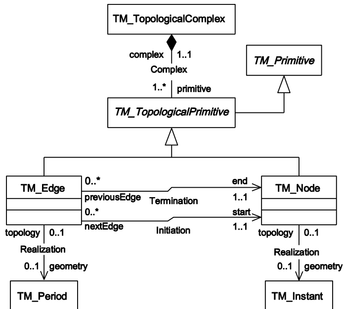
Figure 42 — Profile of temporal topology adapted from ISO 19108
