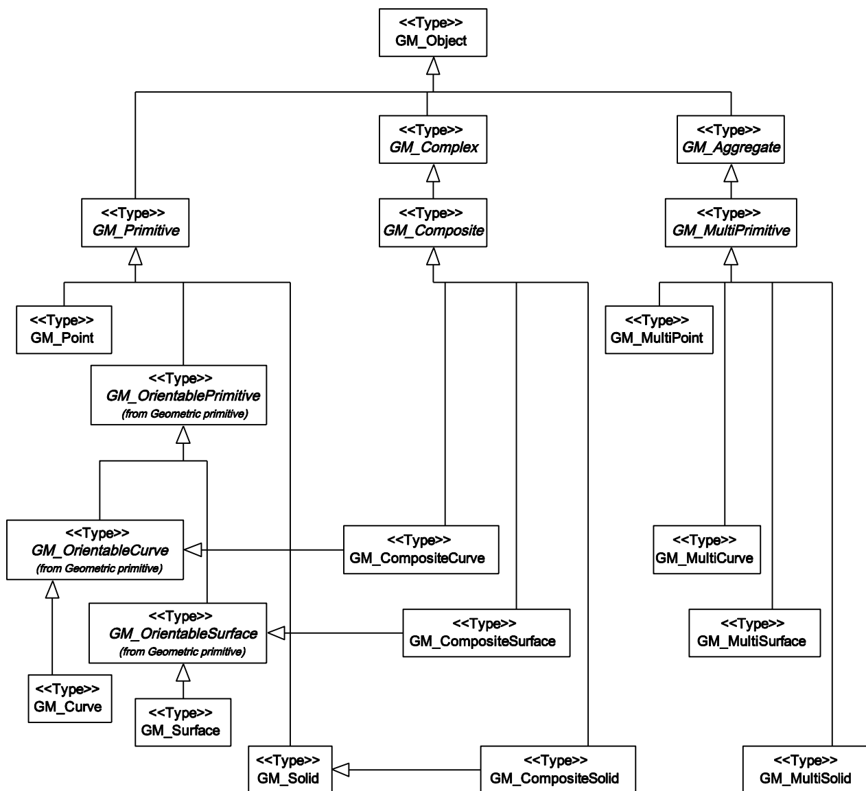
Figure 9 — Implemented subtypes of GM_Object
