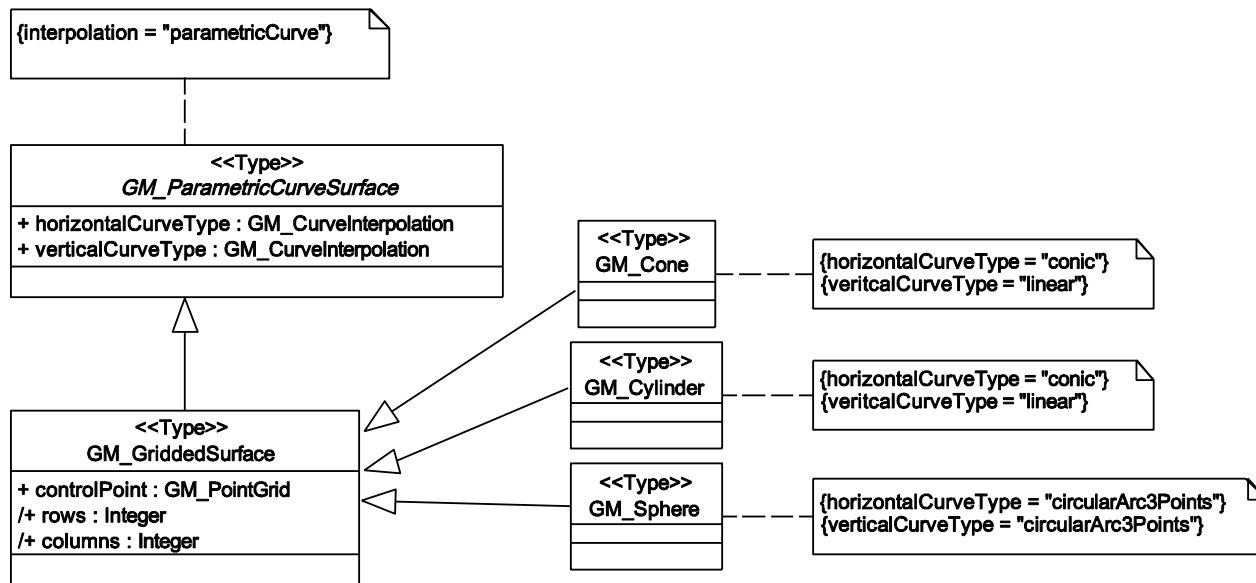
Figure 26 — Gridded surface patches
