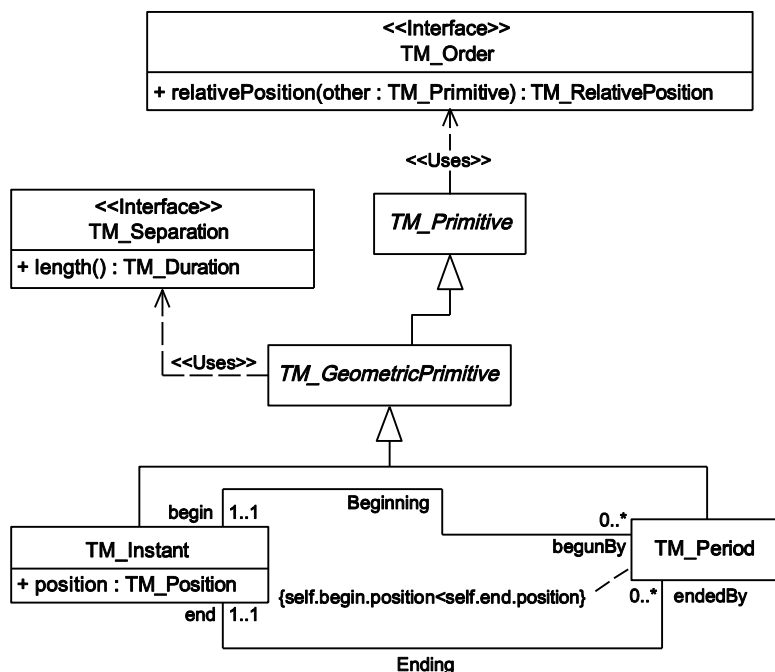
Figure 39 — Profile of temporal geometric objects adapted from ISO 19108
