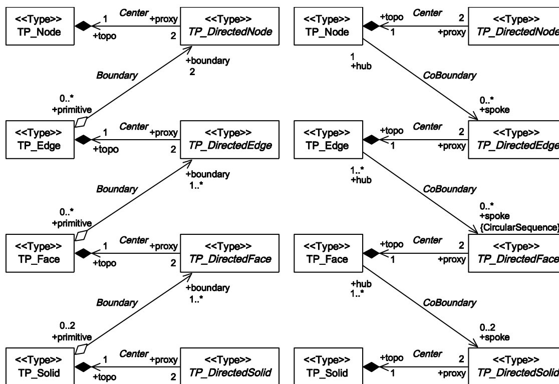
Figure 36 — Boundary and co-boundary relationships
