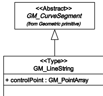
Figure 20 — Line string
