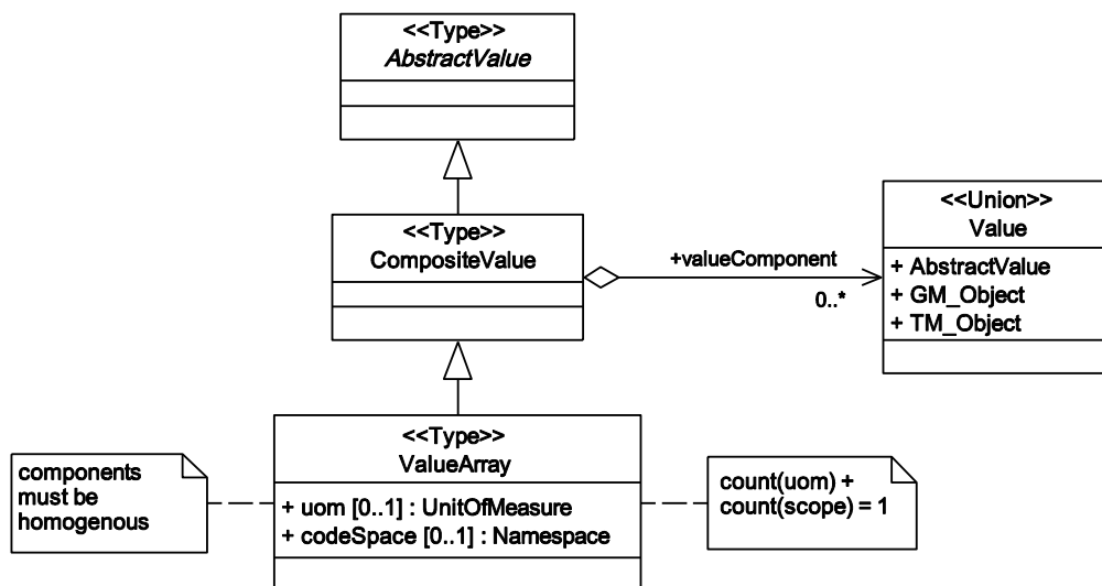
Figure 71 — Composite value
