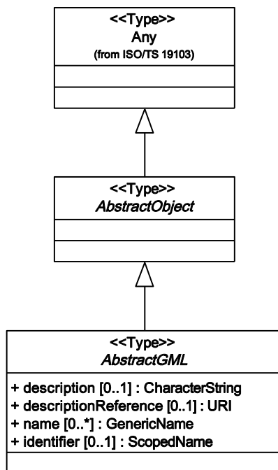
Figure 51 — Base types
