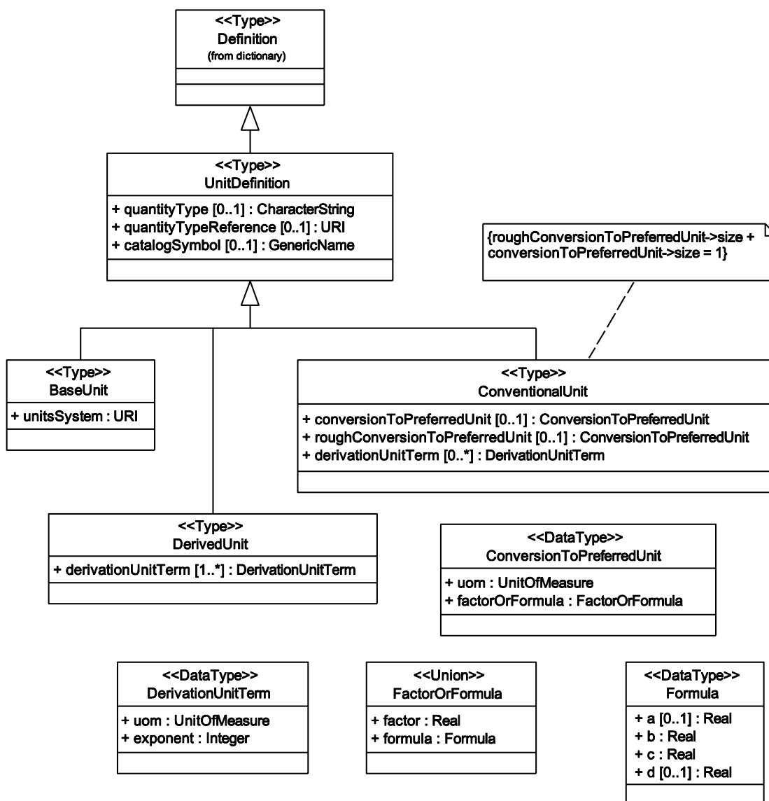
Figure 66 — Unit definitions
