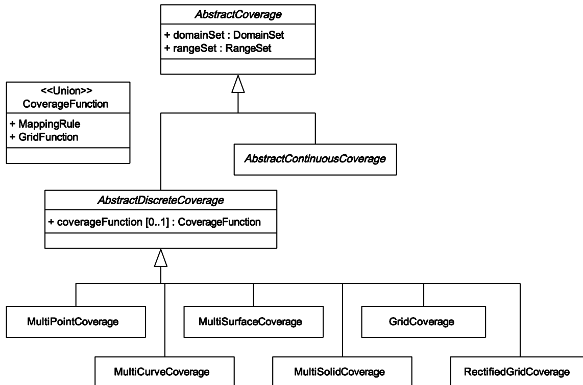
Figure 48 — Discrete coverages
