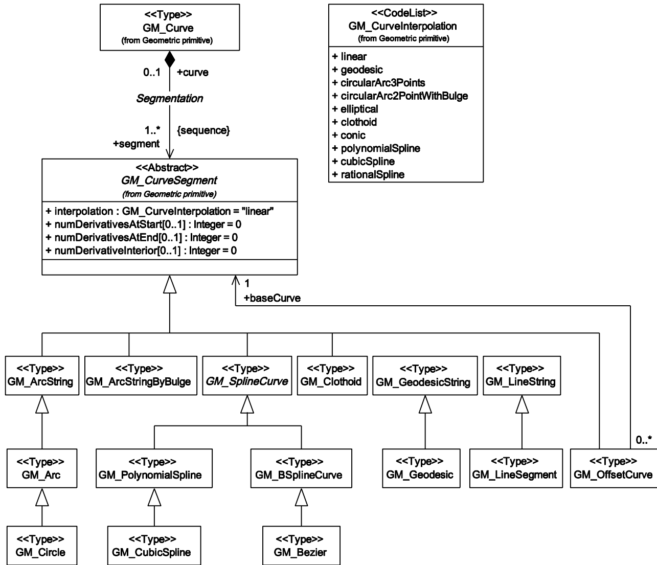
Figure 23 — Curve segments
