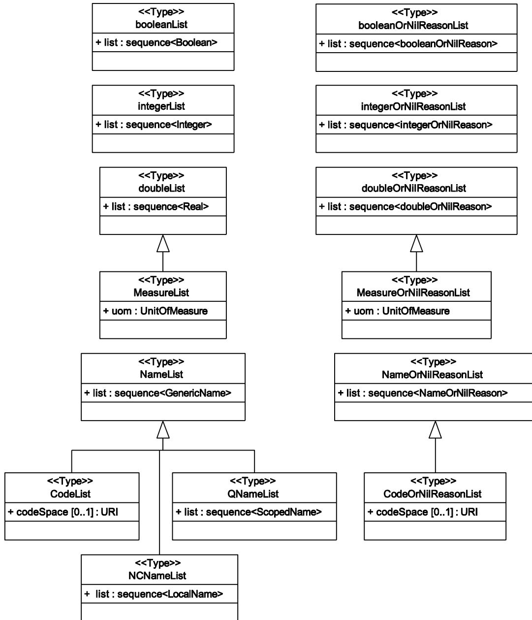
Figure 50 — Lists
