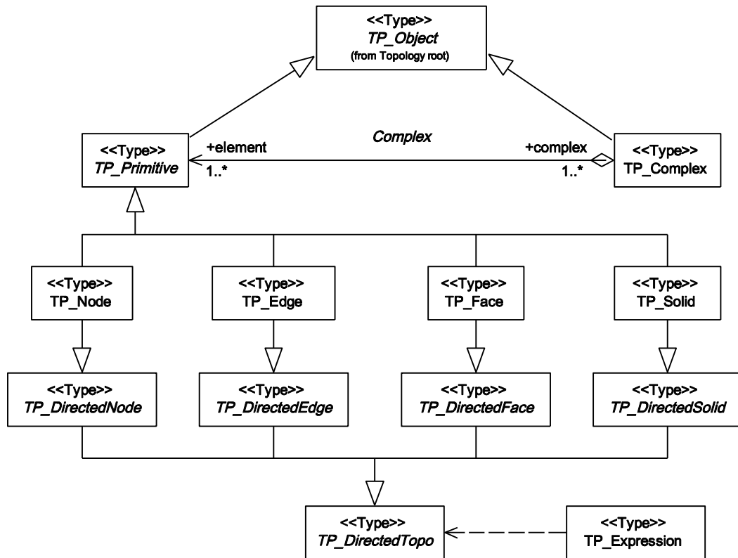
Figure 31 — Topologic primitives
