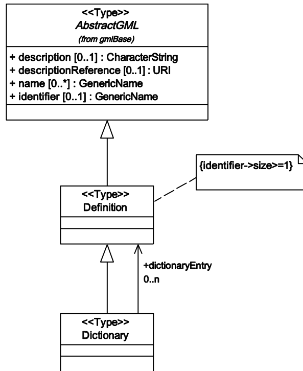
Figure 65 — Dictionaries
