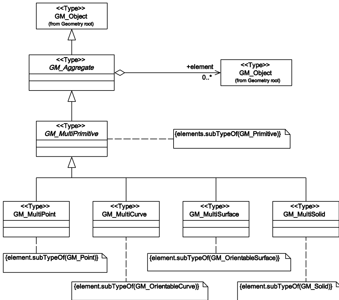
Figure 28 — Geometric aggregates
