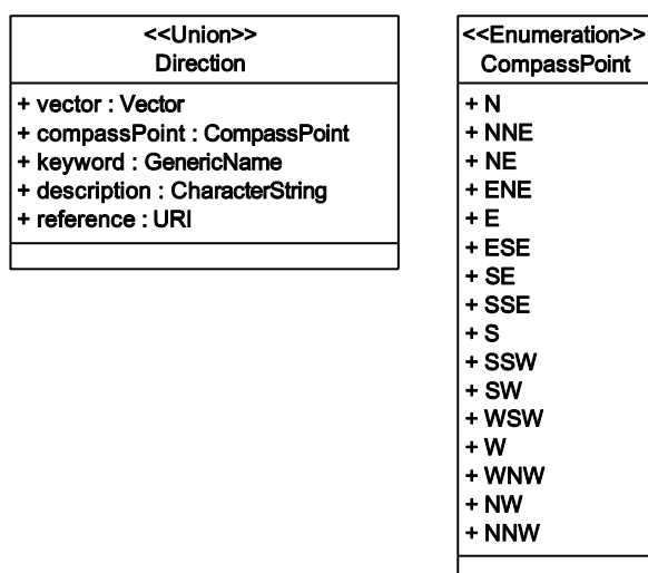
Figure 73 — Direction
