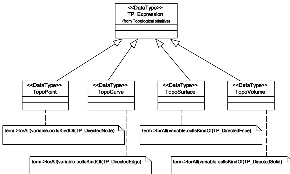
Figure 63 — Topological expressions
