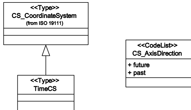
Figure 59 — TimeCS
