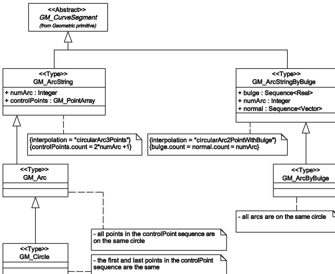
Figure 21 — Arcs and circles
