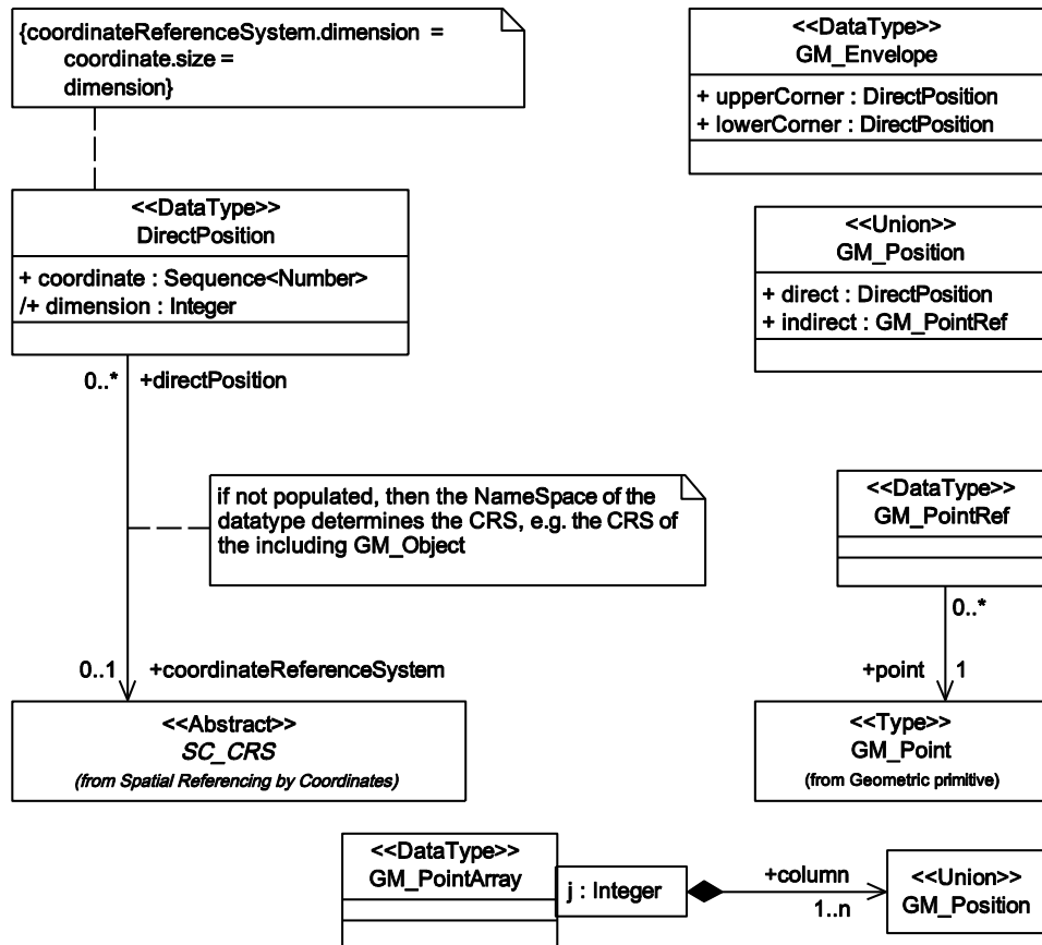
Figure 18 — Coordinate geometry
