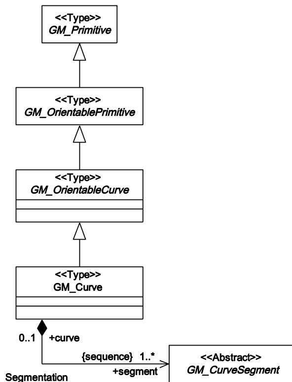
Figure 15 — Curve
