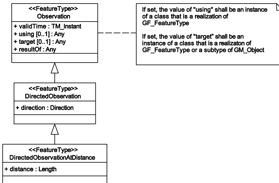
Figure 74 — Observation
