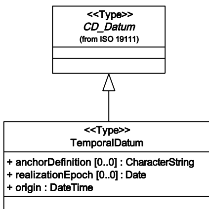
Figure 61 — TemporalDatum
