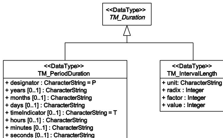
Figure 40 — DataTypes representing temporal duration ISO 19108
