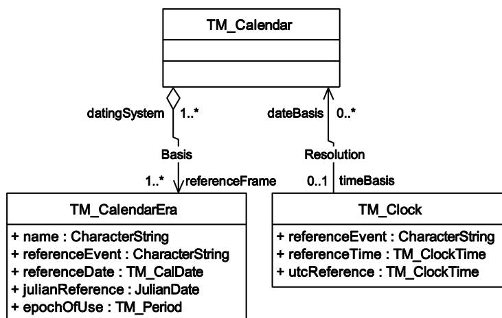
Figure 44 — Model for calendar and clock, from ISO 19108
